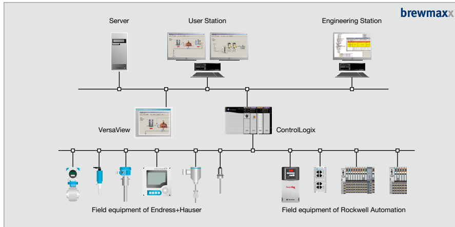
System architecture of the mini-brewery
