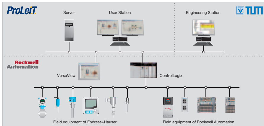
System architecture of the mini-brewery at drinktec 2009, distributed over three booths
